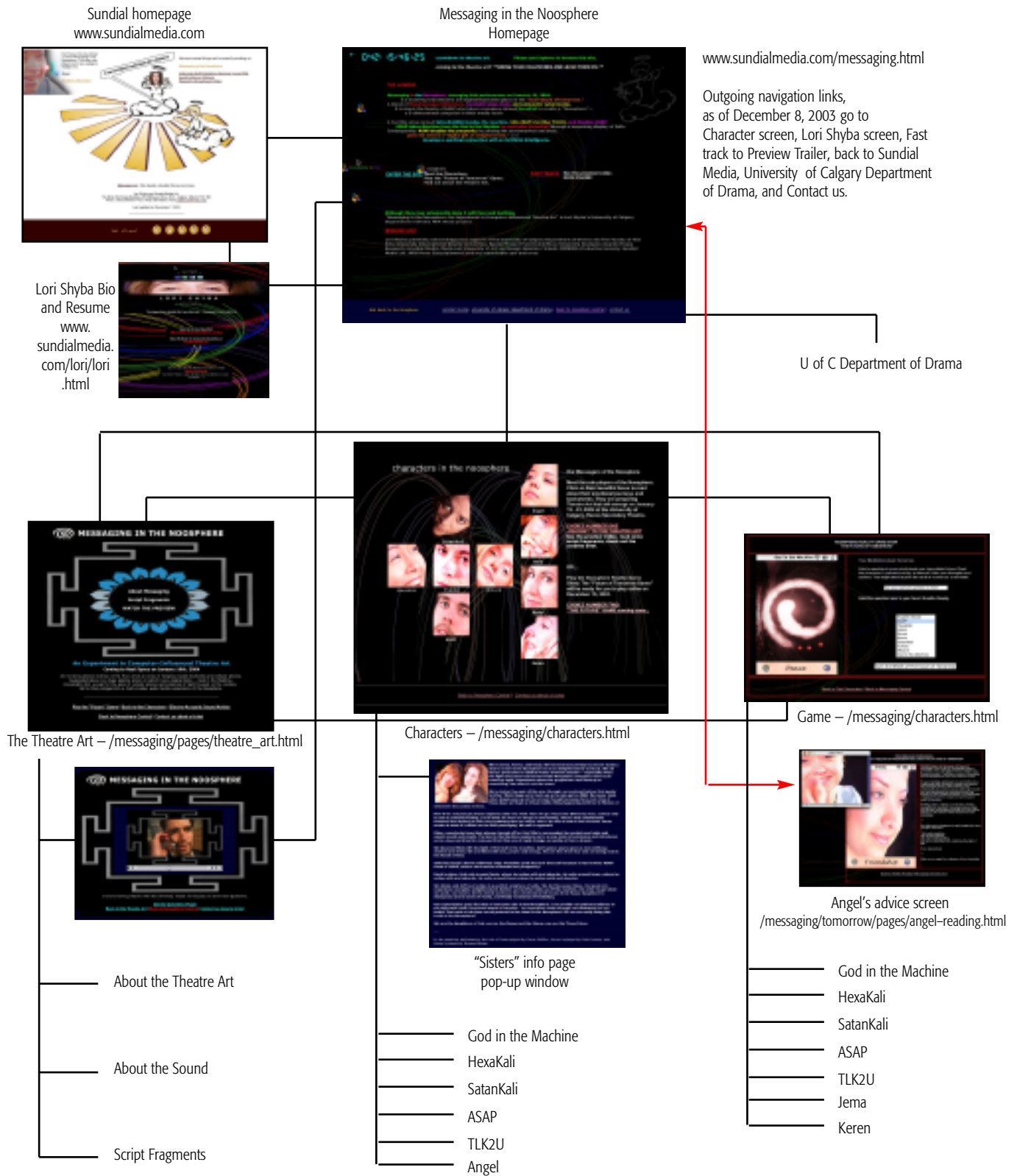
Figure 17 (a). The site map architecture of the completed Web site system.
